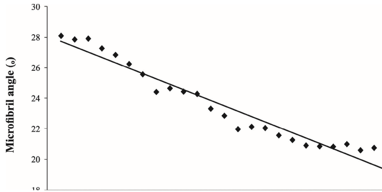
Figure 3. Estimation of the microfibril angle (MFA) of Eucalyptus grandis wood by the cambial age [MFA = 28,1 - 0,35 × a; R 2 = 94,7%].
