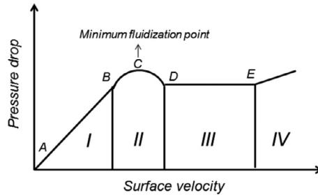
Fig 8. Illustration of the theoretical behavior of pressure loss in fluidized beds, being: I (AB) - static filter bed range, II (B) - bed expansion characterized by the equilibrium between pressure loss and particles weight, C - minimum fluidization point, III (DE) - most of the filter bed in fluidisation, IV - particle drag (adapted from Gupta and Sathiyamoorthy (1999) [4]).
