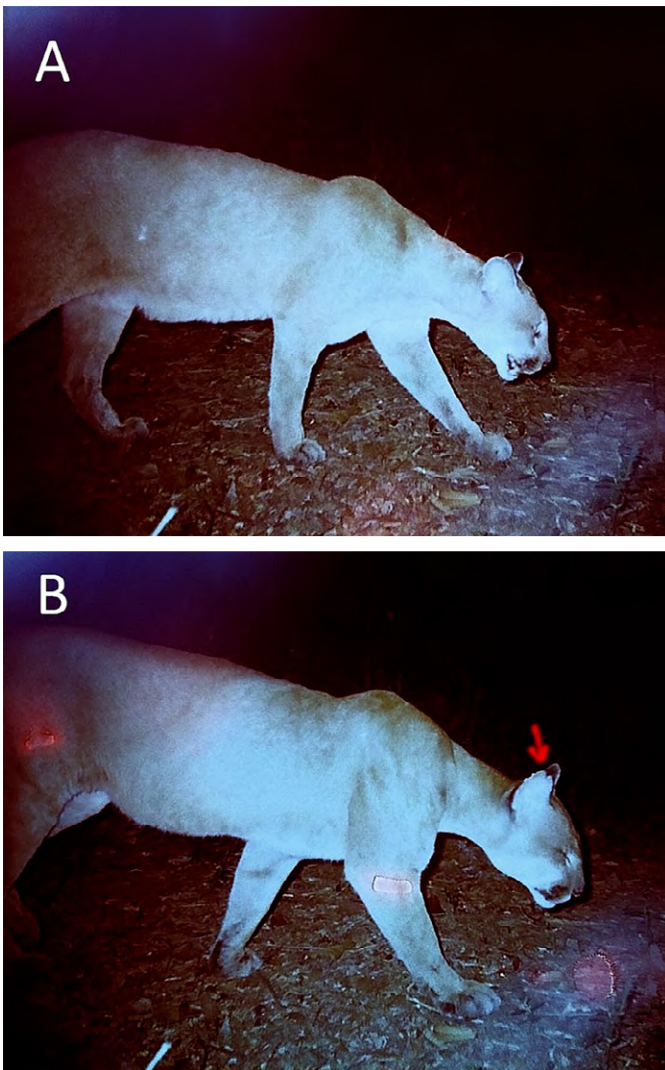
Figure 4. Morphological differences between two individuals of puma ( Puma concolor ) recorded in Quedas do Rio Bonito Ecological Park area: Photograph A was taken by camera trap at 8:46 pm in 6 March 2013, and photograph B was taken at 9:26 pm of the same day.
