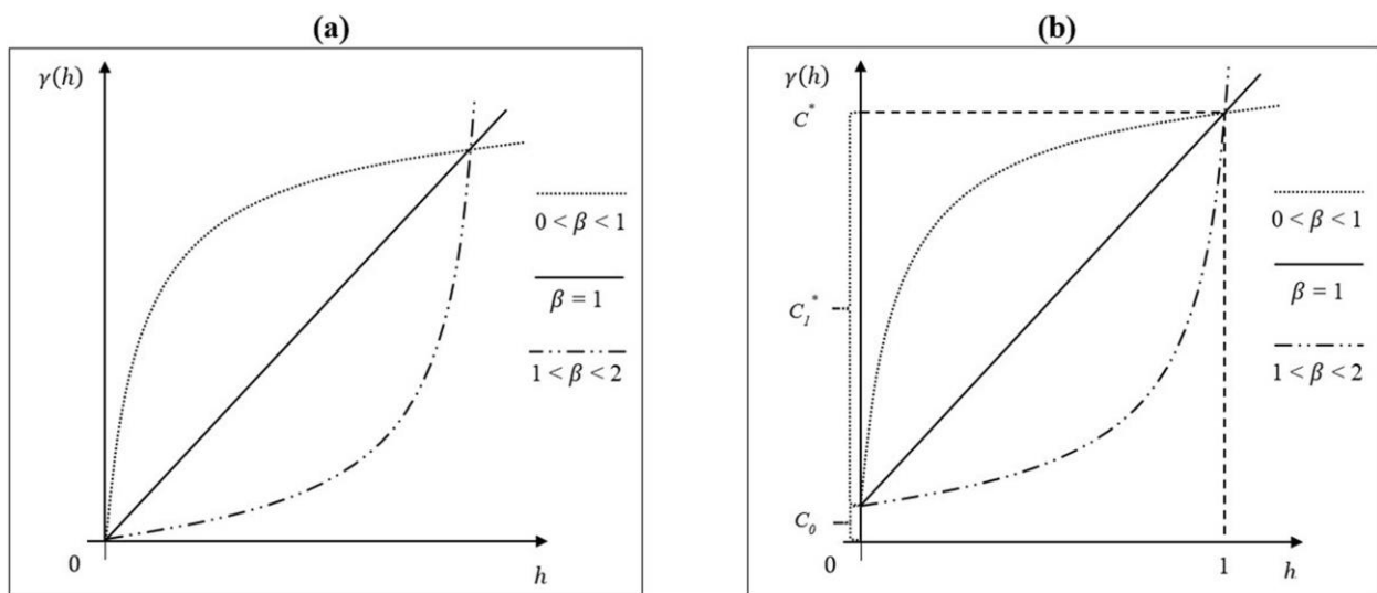
Figure 1: (a) Power semivariogram model; (b) Configuration of the premise in which C_1^* = \alpha .
