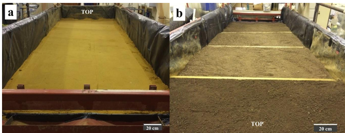
Fig. 2. Soil flume filled with layers of sand (a) followed by soil (b).
