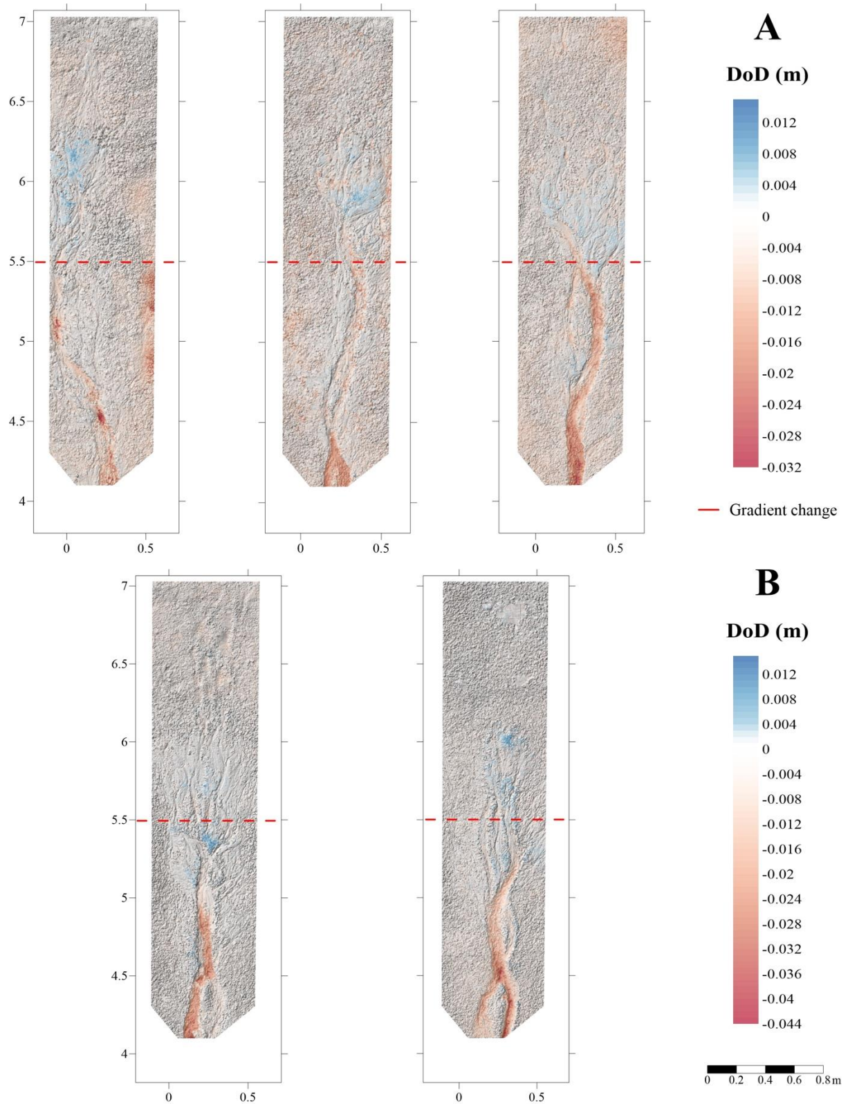
Fig. 6. DEM of difference (DoD) maps, overlain over hillshaded topography, showing rill erosion over runoff at 7 \text{ L min}^{-1} of flow rate in two slopes, 6 % (A) and 9 % (B).
