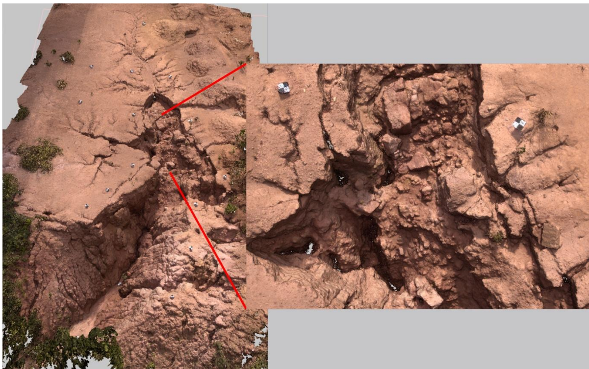
Fig. 5. Dense point cloud showing the 3D reconstruction of complex topographic areas inside the gully.
