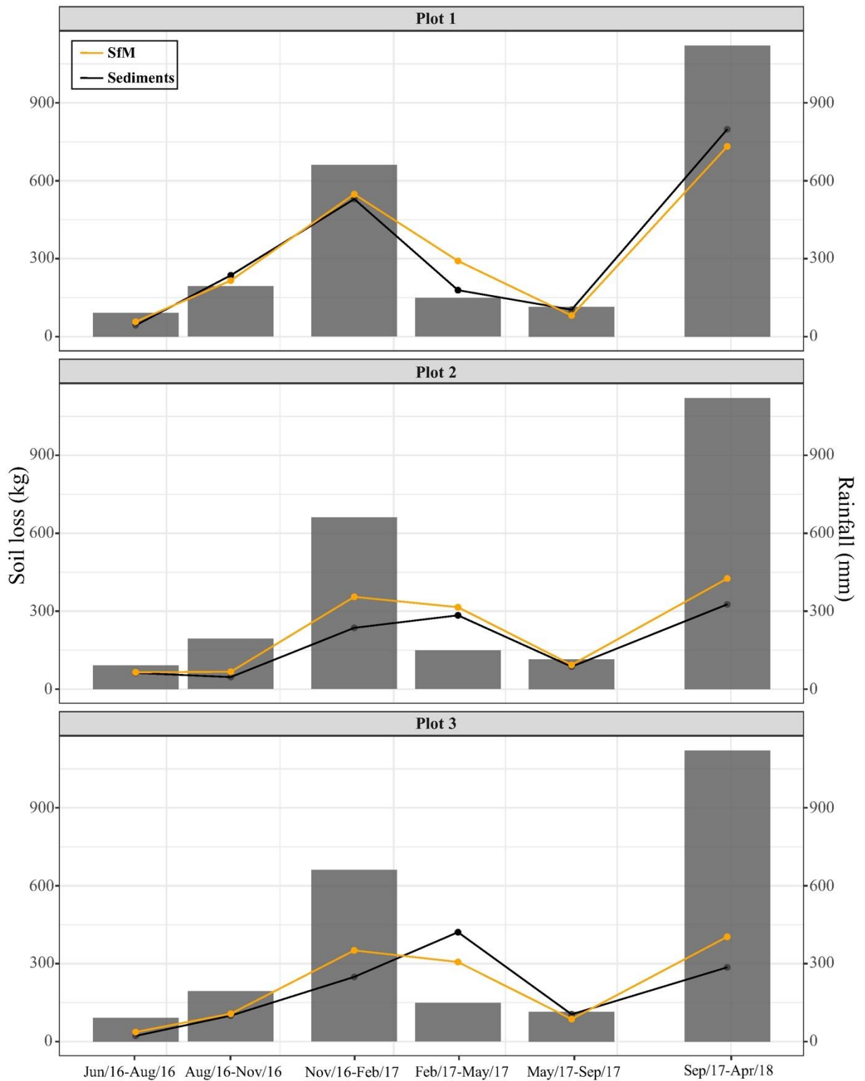
Fig. 6. Soil loss measurements calculated from structure from motion (SfM) and sediment collection for three erosion plots. Lines are to illustrate trend and do not
