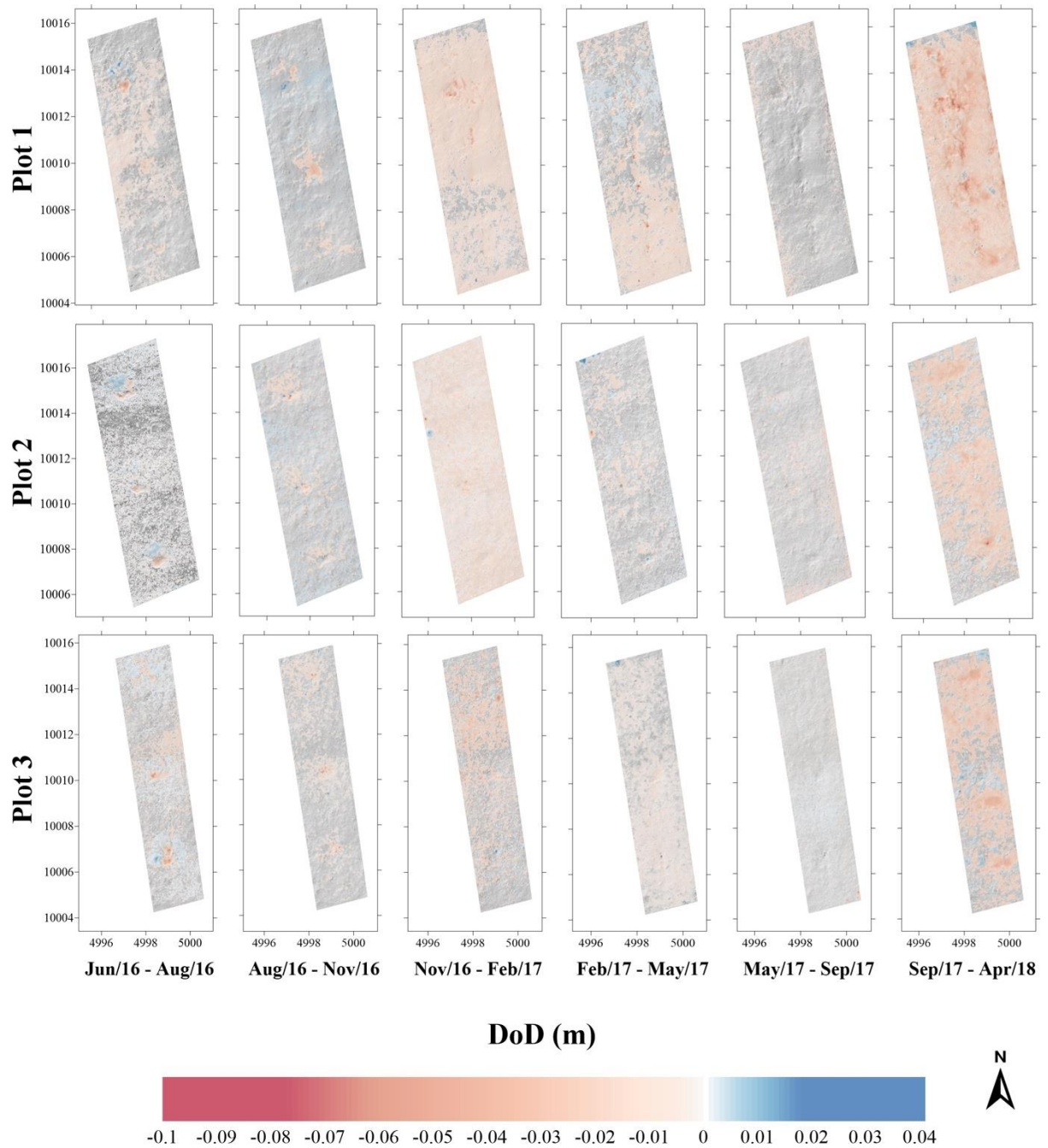
Fig. 4. DEM of difference (DoD) maps, overlain over hillshaded topography, showing soil erosion over natural runoff. Color scale ranges from red (erosion) to blue (deposition). Transparent regions mean no significant changes (DoD is less than the level of detection).
