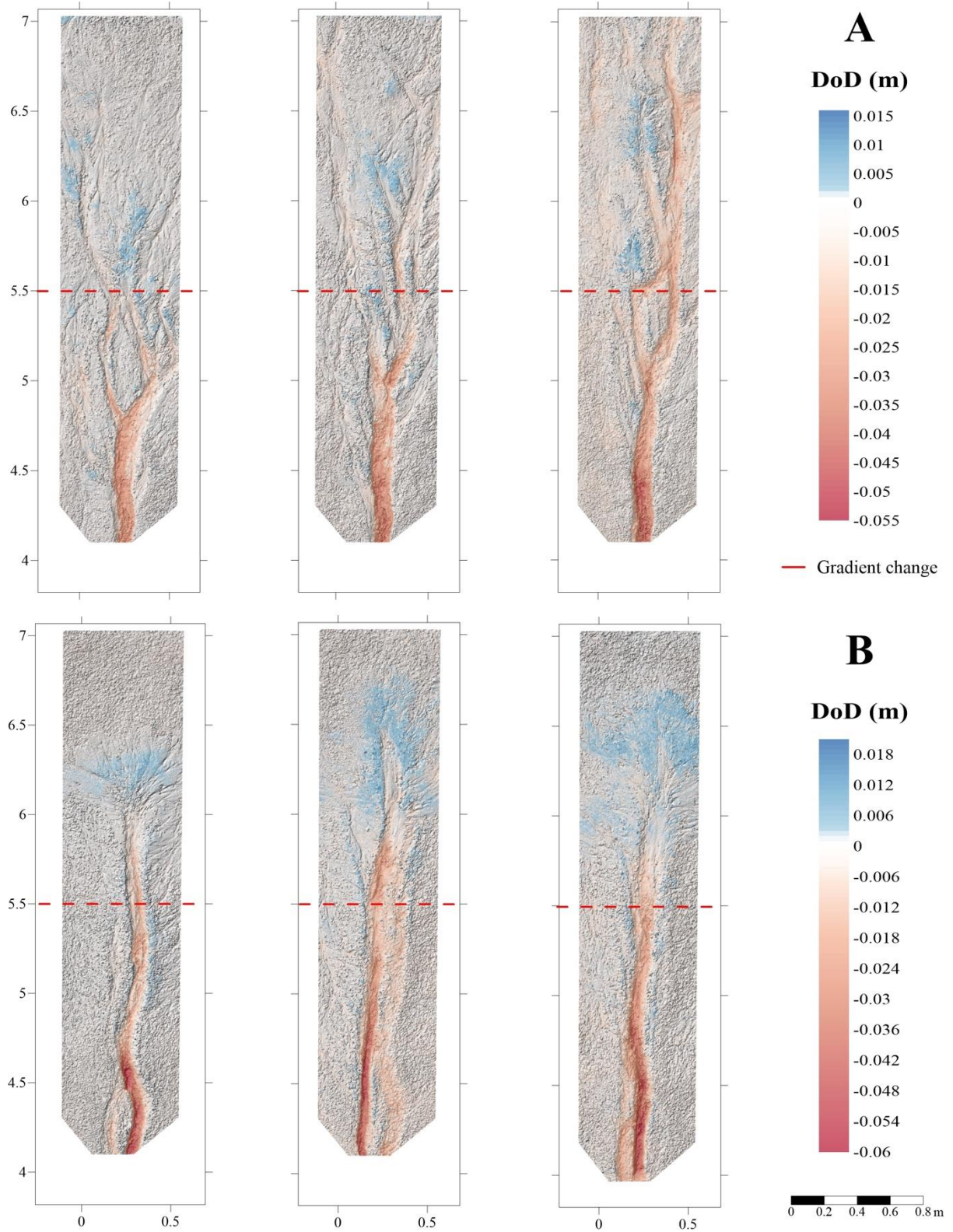
Fig. 7. DEM of difference (DoD) maps, overlain over hillshaded topography, showing rill erosion over runoff at 12 \text{ L min}^{-1} of flow rate in two slopes, 6% (A) and 9% (B).
