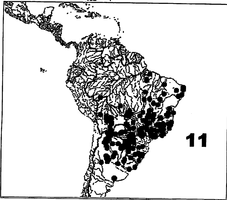
FIGURES 10-11. Distribution maps. 10. Pedaridium ; 11. Trichillum ( Trichillum ).
