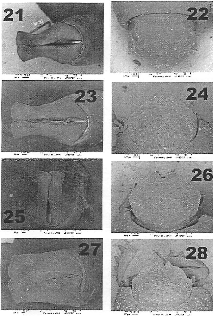
FIGURES 21-28. Dorsal view of head and paramera. 21. Bradypodidium bradyorum ; 22-23. B. alvarengai ; 24-25. B. bustamantei ; 26-27. Eutrichillum arcus ; 28. E. ayri .
