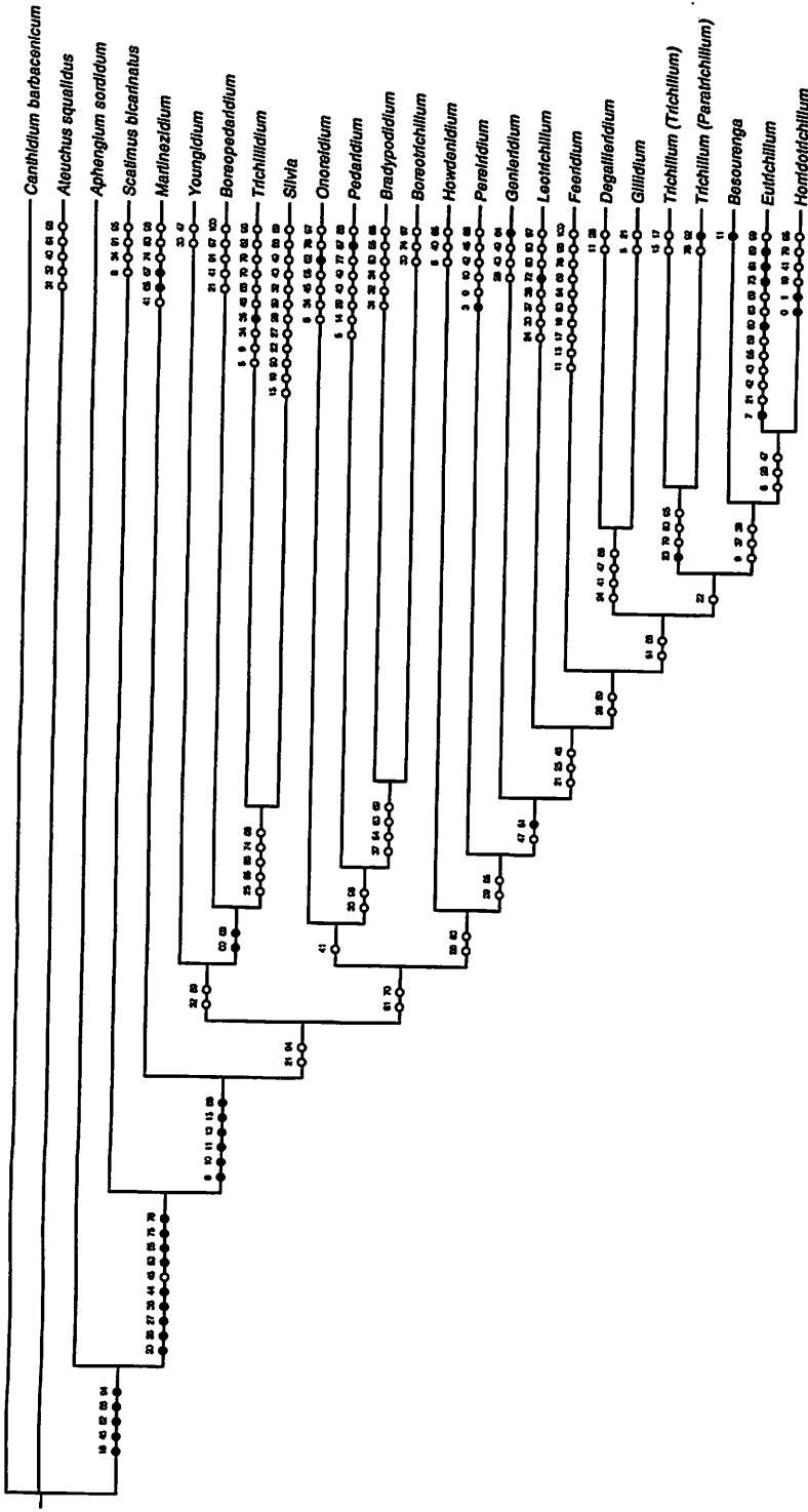
FIGURE 8. Cladogram obtained with PIWe. k=5 , fit=568.5 , 1 of 1; k=6 , fit=591.4 , 1 of 1.
