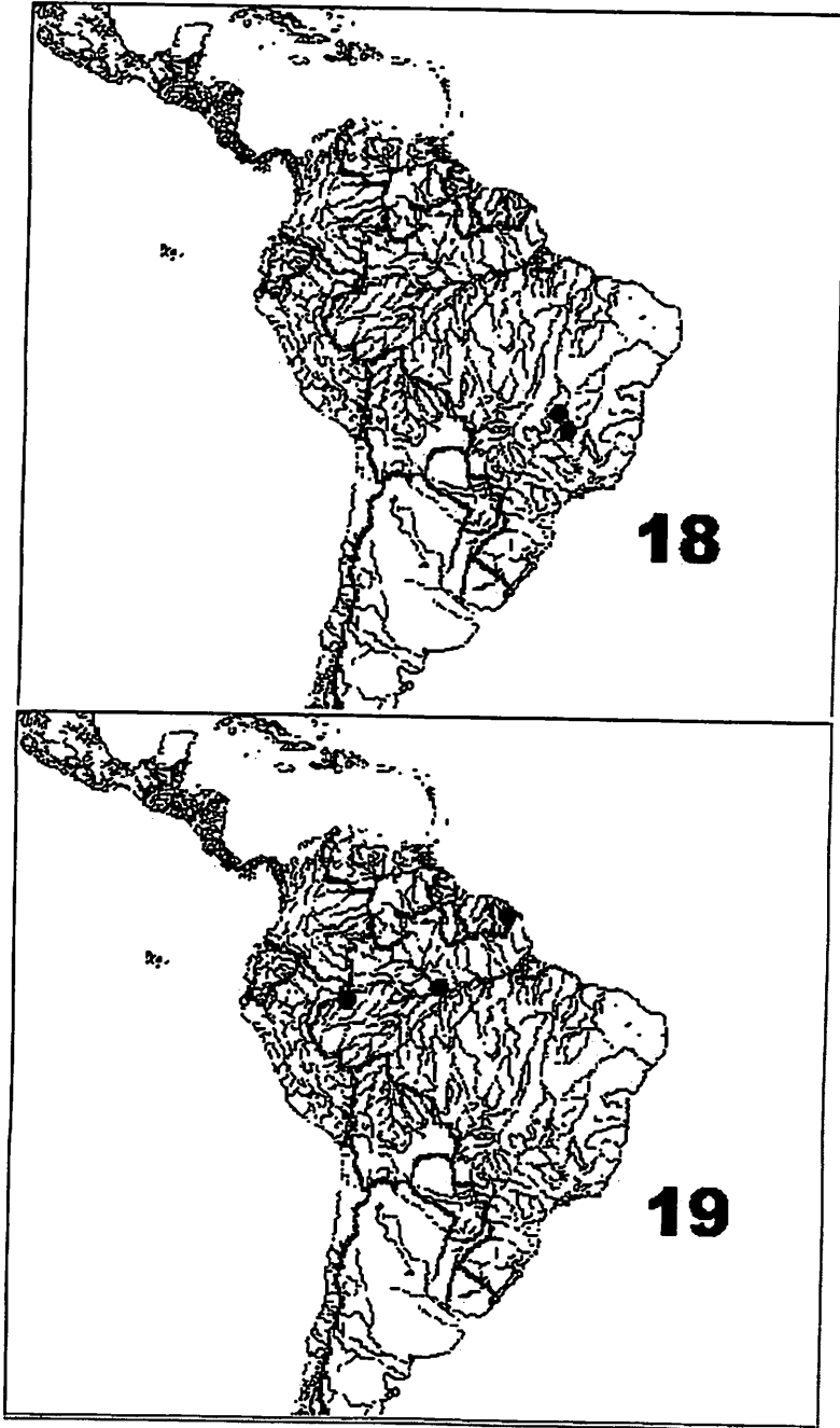
FIGURES 18-19. Distribution maps. 18. Degallieridium ; 19. Feeridium .
