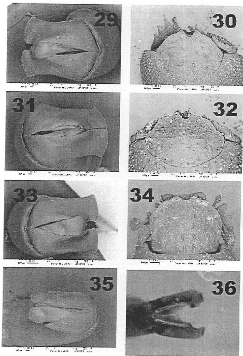
FIGURES 29-36. Dorsal view of head and paramera. 29. Eutrichillum ayri ; 30-31. E. onorei ; 32-33. E. ratcliffei ; 34-35. Leotrichillum leioides ; 36. Martinezidium fulgens .
