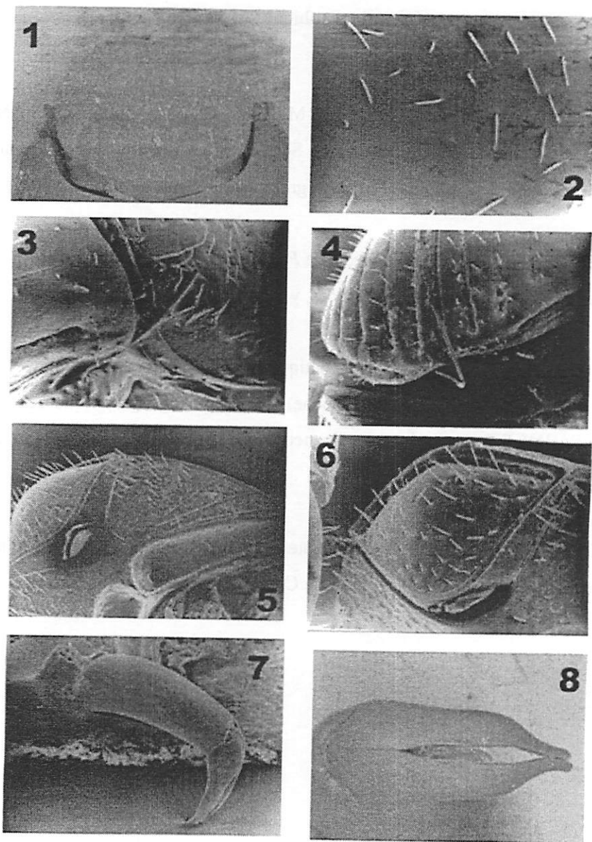
Figs 1-8. Pedaridium maya n. sp. 1. head; 2. punctures on pronotal disc; 3. pronotal hind angle; 4. elytral apex; 5. abdomen, ventral view; 6. pygidium; 7. aedeagus, lateral view; 8. paramera, dorsal view.
