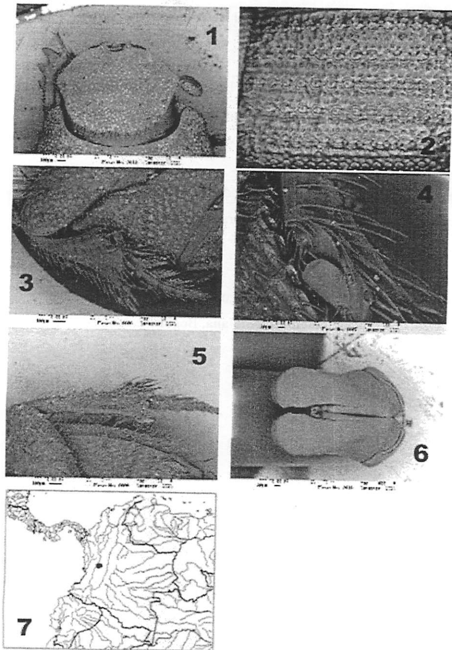
Figs 1-7. Pedaridium medinae n. sp. 1. head; 2. elytron; 3. male hind tibia; 4. same, detail; 5. female hind tibia; 6. male genitalia, dorsal view; 7. distribution in Colombia.
