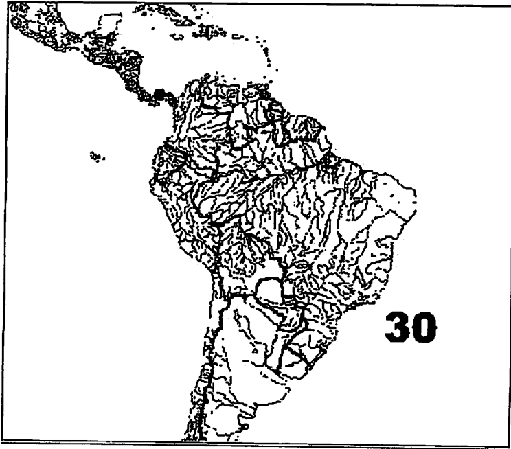
FIGURE 30. Distribution map for Youngidium .
