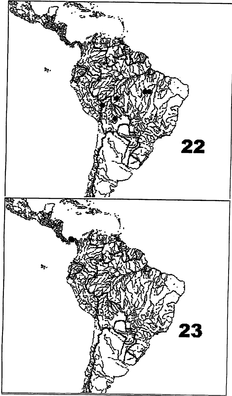
FIGURES 22-23. Distribution maps. 22. Horridotrichillum ; 23. Howdenidium .
