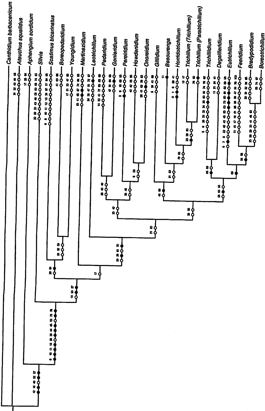
FIGURE 4. Cladogram obtained with PiWe. k=1 , fit=349.8 , 3 of 4.
