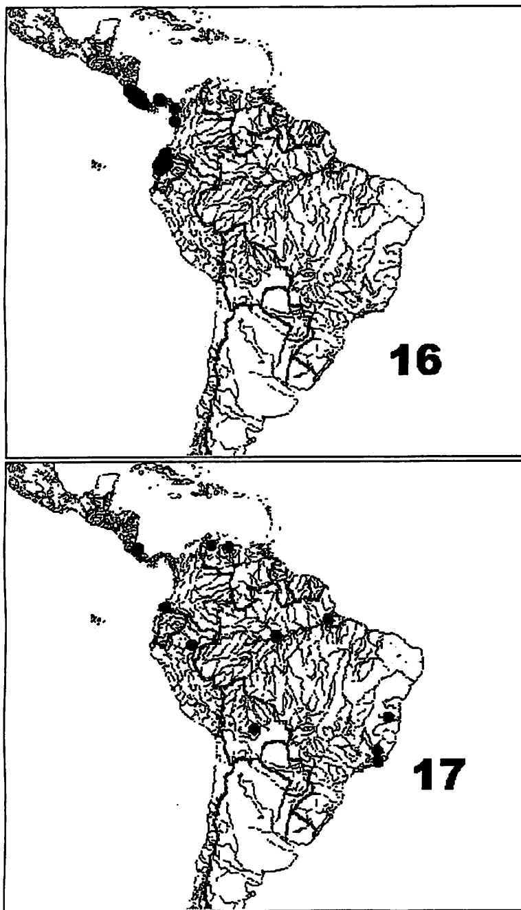
FIGURE 16-17. Distribution maps. 16. Boreotrichillum ; 17. Bradypodium .
