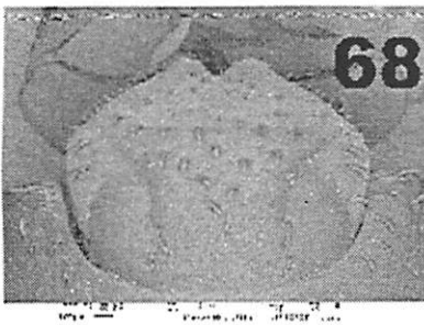
FIGURES 62-68. Dorsal view of head. 62. Howdenidium bottimeri ; 63. Youngidium brevisetosum ; 64. Boreotrichillum pilosum ; 65. Leotrichillum louzadaorum ; 66. Gillidium gilli ; 67. Degallieridium liliputanum ; 68. Feeridium woodruffi .
