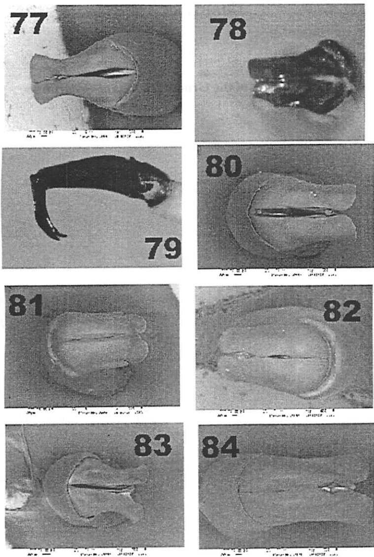
FIGURES 77-78, 80-84. Dorsal view of paramera; 79. lateral view of aedeagus. 77. Bradypodidium adisi ; 78. Howdenidium bottimeri ; 79. Youngidium brevisetosum ; 80. Boreotrichillum pilosum ; 81. Leotrichillum louzadaorum ; 82. Genieridium cryptops ; 83. Degallieridium liliputanum ; 84. Feeridium woodruffi .
