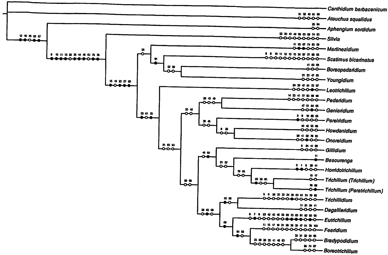
FIGURE 2. Cladogram obtained with PiWe. k=1, fit=349.8, 1 of 4.
