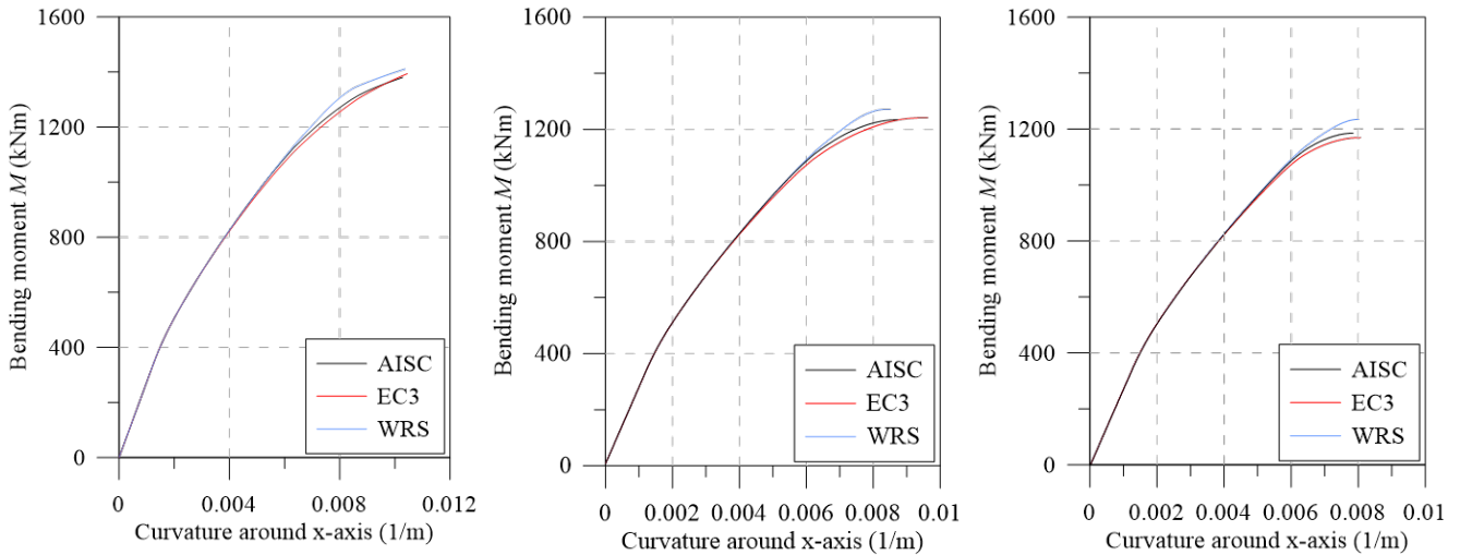
(a) For N = 4000 kN and \gamma = 0
