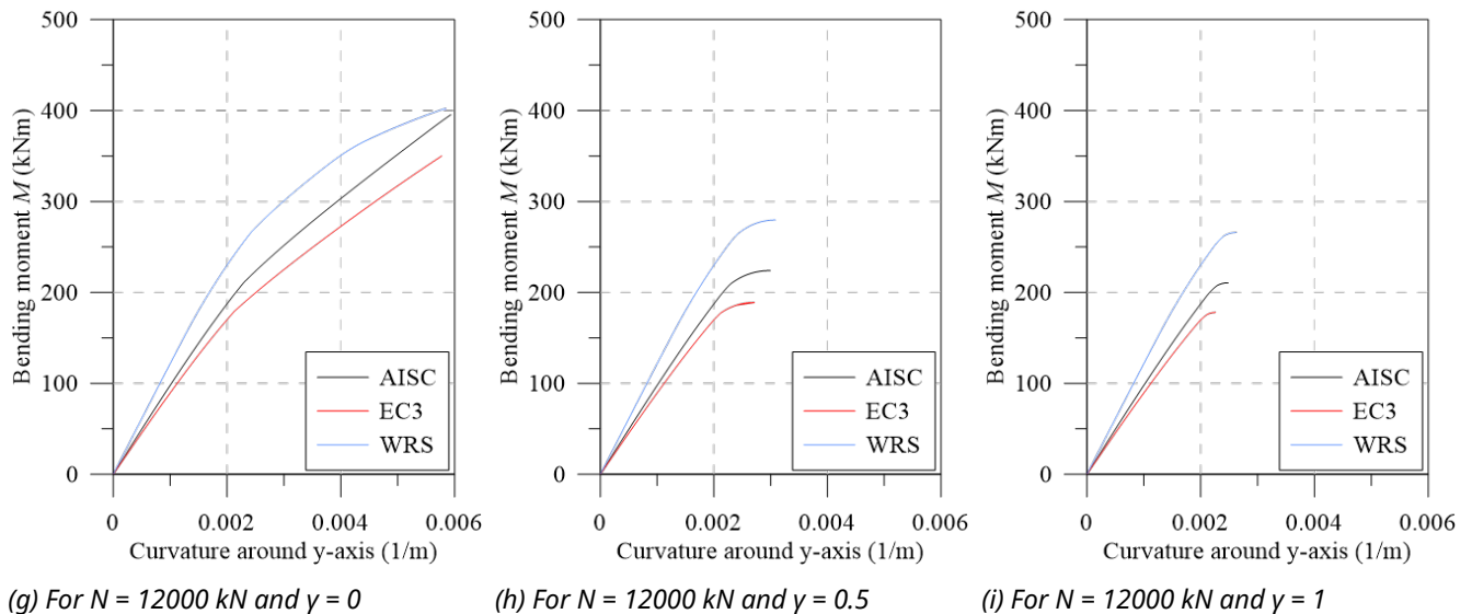
Figure 16 Influence of concrete softening parameter \gamma in minor axis bending
