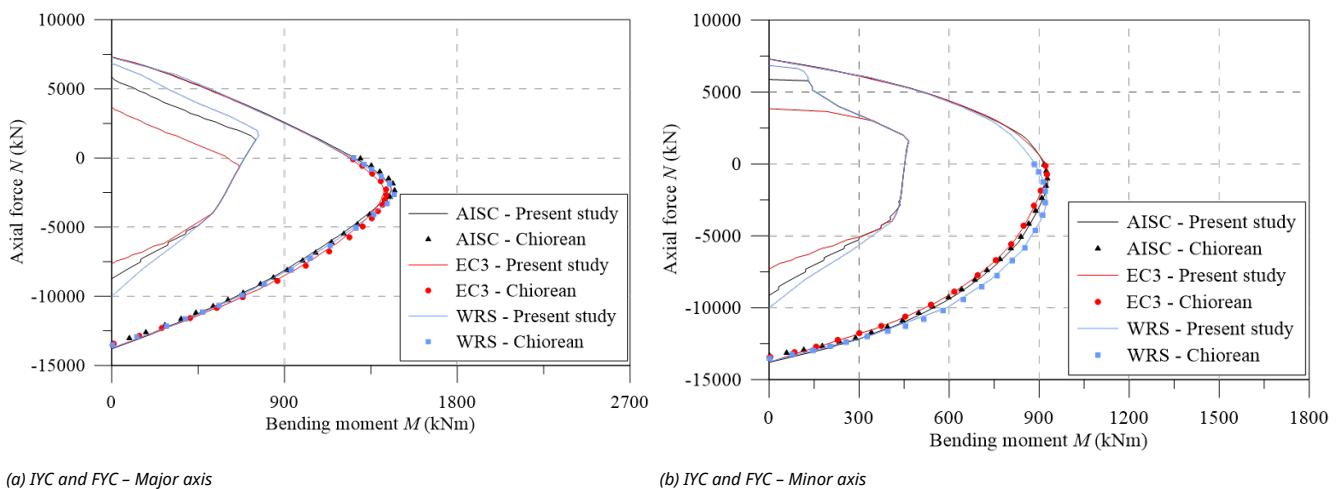
Figure 14 Yield curves of composite section.
