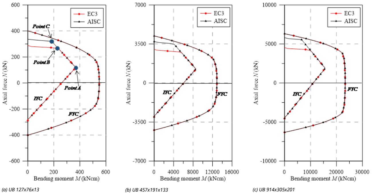
Figure 8 Yield curves for UB sections - major axis bending.
