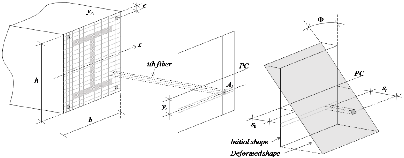
Figure 5 Linear strains field around x axis.
