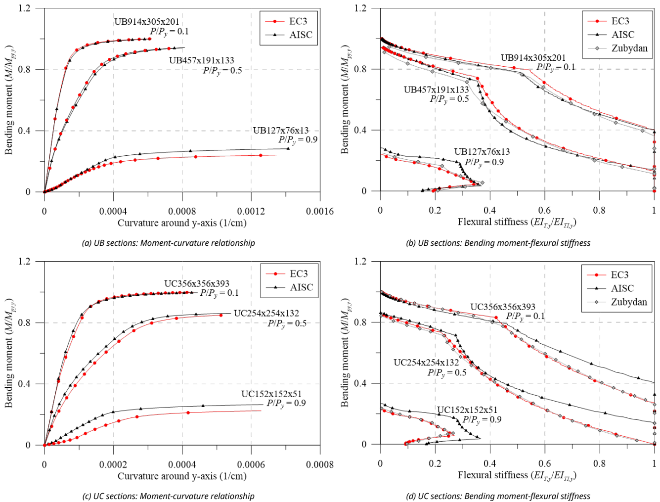
Figure 7 Steel UB and UC non-linear behavior.
