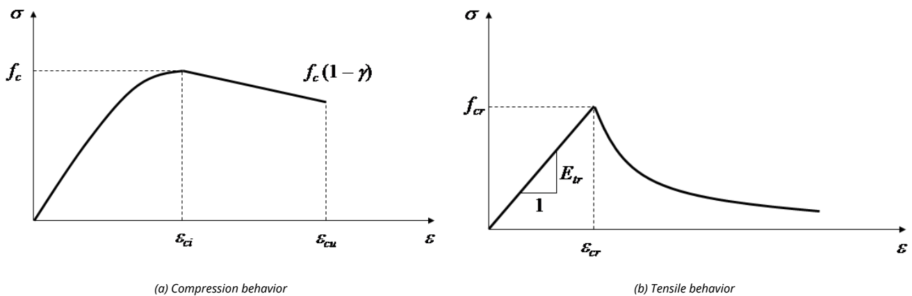
Figure 4 Concrete constitutive relationship.
