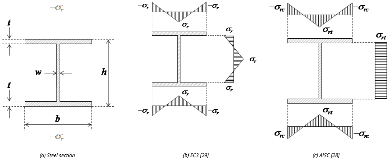
Figure 2 Design codes models to describe the residual stresses.
