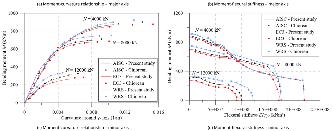
Figure 13 Analysis of steel-concrete composite section.
