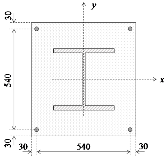
Figure 12 W12x120 section totally encased in concrete (dimensions in mm).
