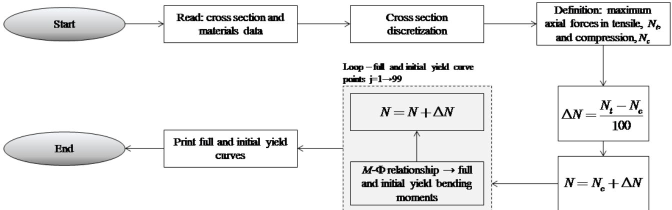
Figure 6 Flowchart for obtaining the interaction curves.
