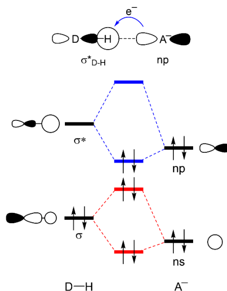
Scheme 2.1 – Generic MO diagram of DH\cdots A^- hydrogen bonds ( D, A = \text{halogen} ). Orbital interactions in blue and Pauli repulsion in red (WOLTERS; BICKELHAUPT, 2012).
