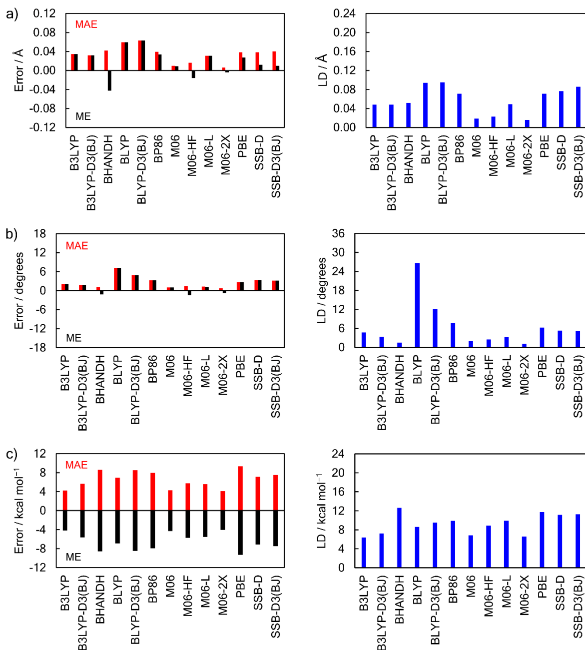
Figure 3.6. Mean absolute error (MAE, red), mean error (ME, black), and largest deviation (LD, blue) of the ZORA-DFT/QZ4P functionals relative to the ZORA-CCSD(T)/BS3+ a) Ch \cdots A ^- bond lengths, b) bond angles \Theta_2 , and c) D_2\text{Ch}\cdots\text{A}^- counterpoise-corrected complexation energies.
