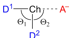
Scheme 4.1. Chalcogen-bonded D 2 Ch•••A − model complexes (Ch = O, S, Se, Te; D, A = F, Cl, Br).
