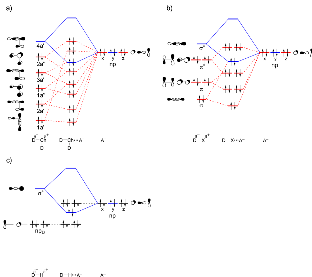
Figure 4.8. Generic molecular orbital diagrams for a) D 2 Ch...A - chalcogen bonds, b) DX...A - halogen bonds, and c) DH...A - hydrogen bonds.
