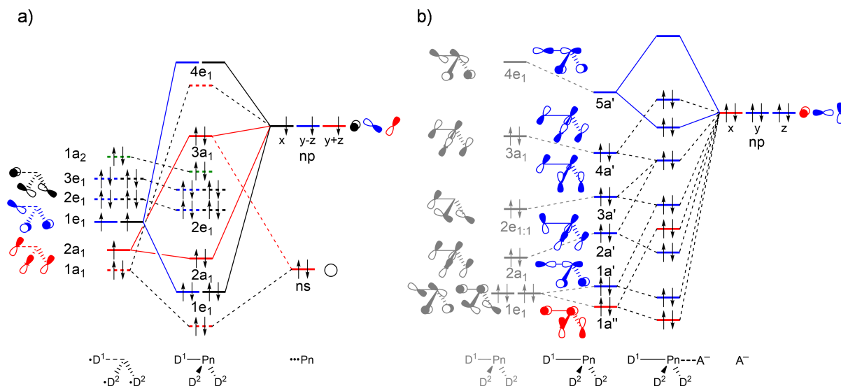
Fig. 5.2. Schematic molecular orbital diagram for (a) isolated D_3Pn fragments at C_{3v} symmetry (red: a_1 ; green: a_2 ; blue: e_{1:1} ; black: e_{1:2} ) and (b) D_3Pn \cdots A^- complexes. The first column in (b) refers to the isolated D_3Pn fragment and the second column refers to the D_3Pn fragment deformed to its C_s symmetric geometry in the complex (blue: a' ; red: a'' ), in which one D–Pn bond has been elongated. See Appendix 5.3 for computed 3D isosurfaces of the orbitals.
