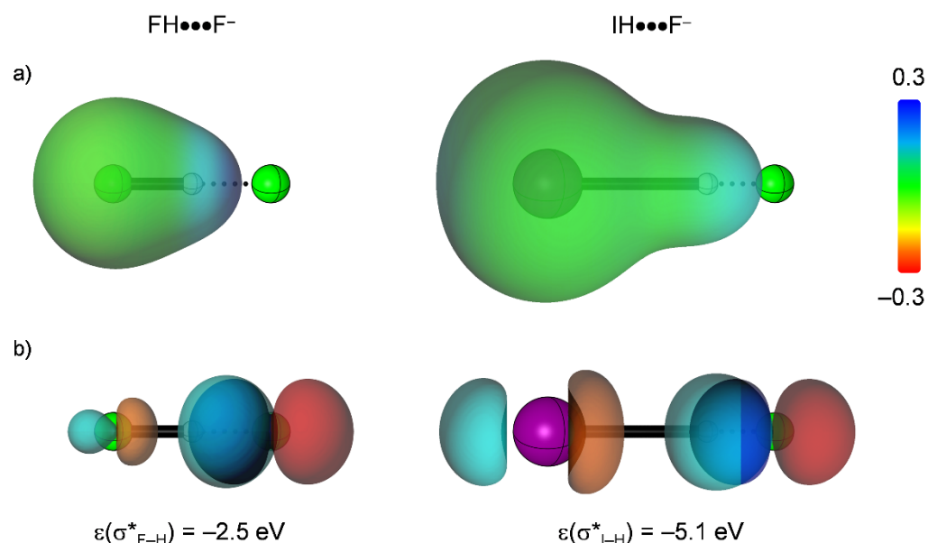
Figure 2.4 – a) Molecular electrostatic potential of the DH fragment at 0.01 a.u. (blue, positive; red, negative; see color scale) and b) HOMO–LUMO interactions within the DH\cdots F^- hydrogen bonded complexes (D = F, I; F, green; I, purple; H, white) computed at ZORA-BP86/TZ2P level. This is a reproduction of the results from Wolters and Bickelhaupt (WOLTERS; BICKELHAUPT, 2012).
