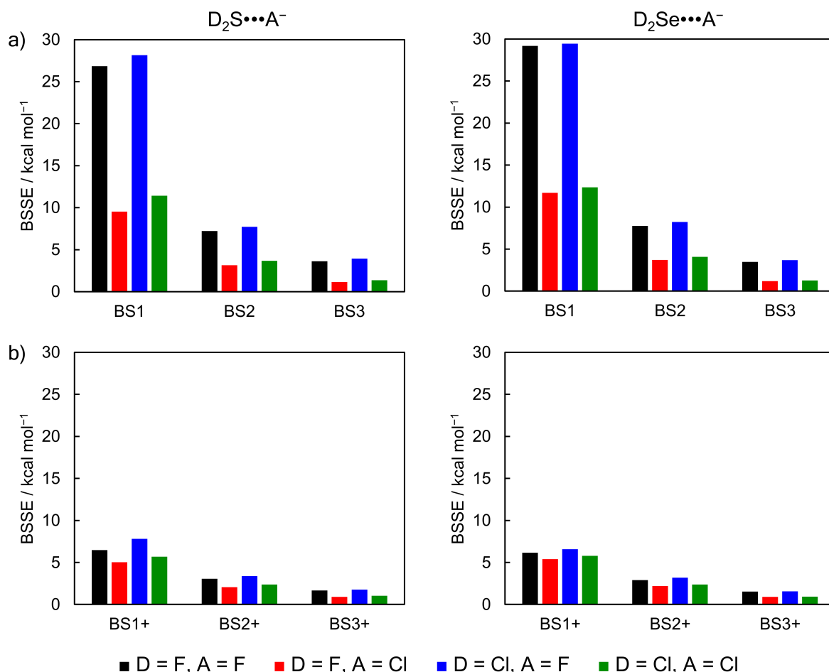
Figure 3.4. Basis set superposition error (BSSE) calculated at ZORA-CCSD(T) level for \text{D}_2\text{Ch}\cdots\text{A}^- chalcogen-bonded complexes along a) BS1 to BS3 and b) BS1+ to BS3+ basis sets.
