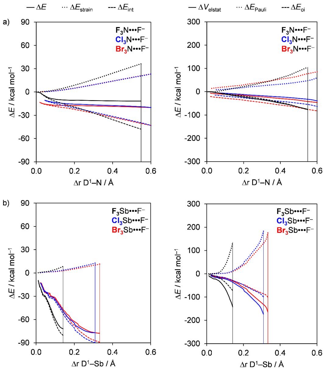
Fig. 5.6. Activation strain (left panel) and energy decomposition (right panel) analyses of (a) D_3N \cdots F^- and (b) D_3Sb \cdots F^- (black, D = F ; blue, D = Cl ; red, D = Br ). The vertical lines indicate the position of the stationary points.
