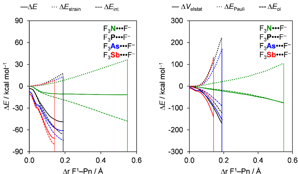
Fig. 5.1. Activation strain (left panel) and energy decomposition (right panel) analyses of F_3Pn\cdots F^- pnictogen-bonded complexes (green, Pn = N ; black, Pn = P ; blue, Pn = As ; red, Pn = Sb ). The vertical lines indicate the position of the stationary points.
