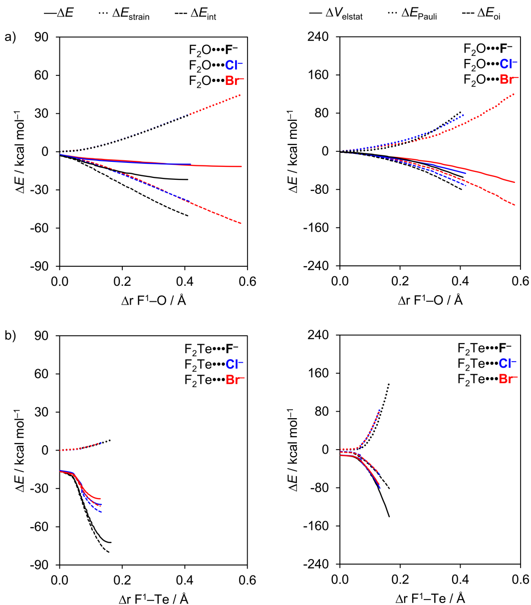
Figure 4.6. Activation strain (left panel) and energy decomposition (right panel) analyses of a) \text{F}_2\text{O} \cdots \text{A}^- and b) \text{F}_2\text{Te} \cdots \text{A}^- (black, \text{A}^- = \text{F}^- ; blue, \text{A}^- = \text{Cl}^- ; red, \text{A}^- = \text{Br}^- ).
