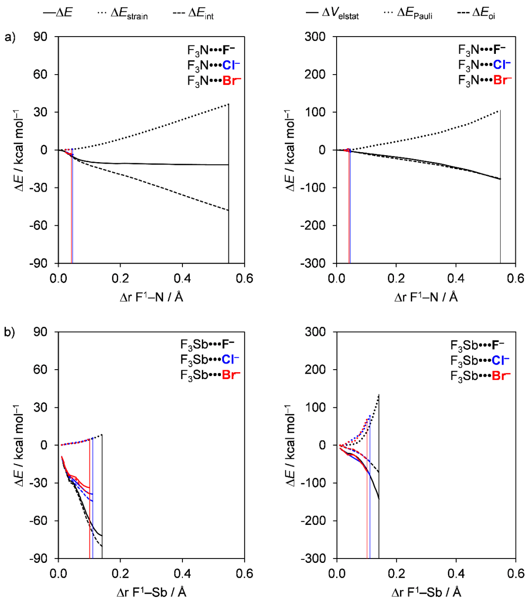
Fig. 5.5. Activation strain (left panel) and energy decomposition (right panel) analyses of (a) \text{F}_3\text{N}\cdots\text{A}^- and (b) \text{F}_3\text{Sb}\cdots\text{A}^- (black, \text{A}^- = \text{F}^- ; blue, \text{A}^- = \text{Cl}^- ; red, \text{A}^- = \text{Br}^- ). The vertical lines indicate the position of the stationary points.
