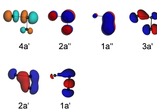
Appendix 4.3. Schematic FMO and DFT MO isosurfaces (at 0.04 a.u.) for the \text{D}_2\text{Ch} fragment in a) the ground state at C_{2v} symmetry and in b) the geometry of the complex at C_s symmetry, computed at ZORA-M06/QZ4P.
