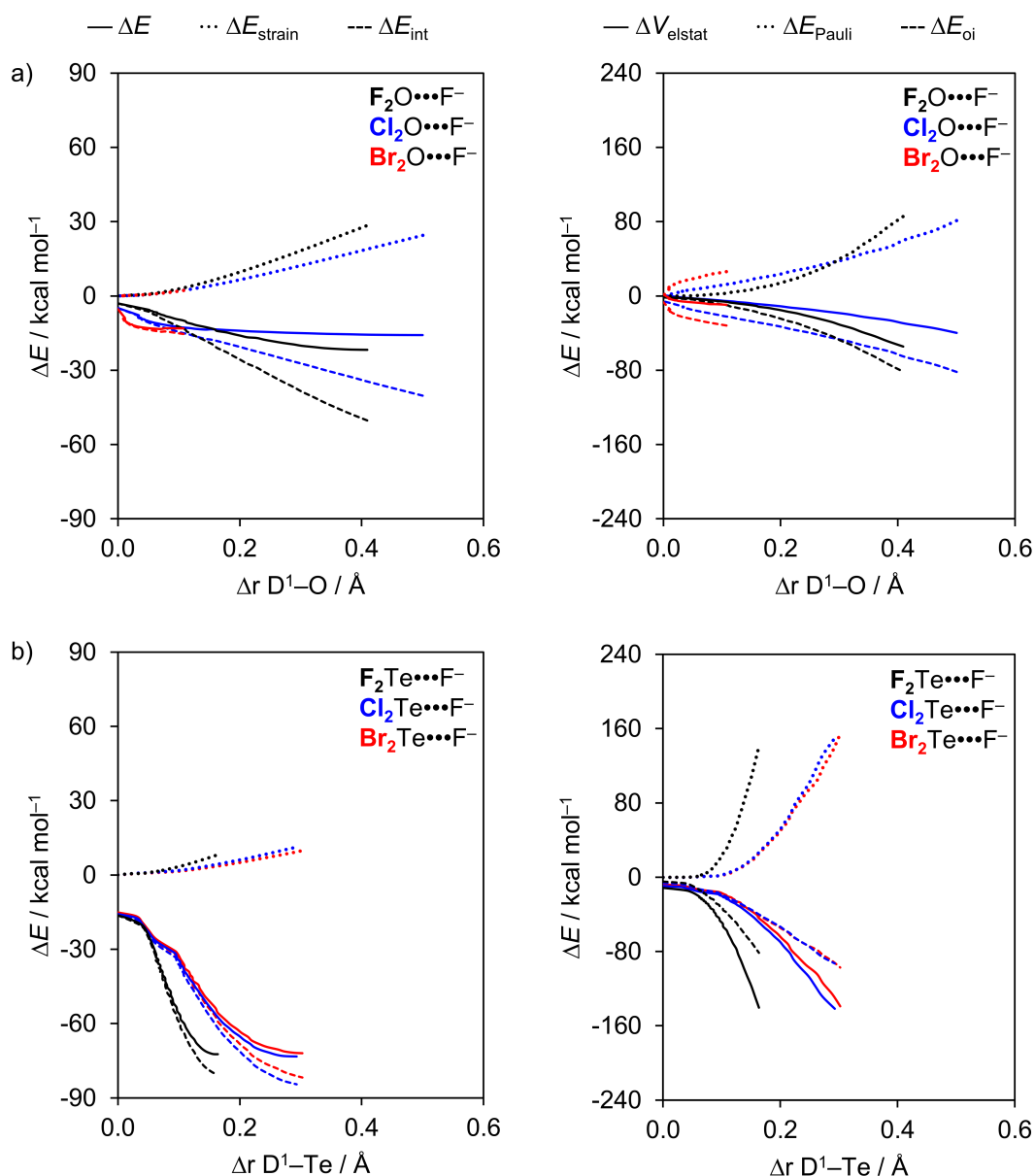
Figure 4.7. Activation strain (left panel) and energy decomposition (right panel) analyses of a) \text{D}_2\text{O}\cdots\text{F}^- and b) \text{D}_2\text{Te}\cdots\text{F}^- (black, D = \text{F} ; blue, D = \text{Cl} ; red, D = \text{Br} ).
